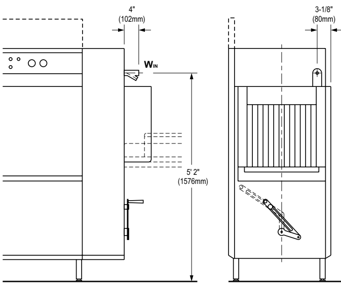
Incoming water supply connection (3/4" NPT) For location of electrical supply connection, refer to the dishwasher spec sheet.
