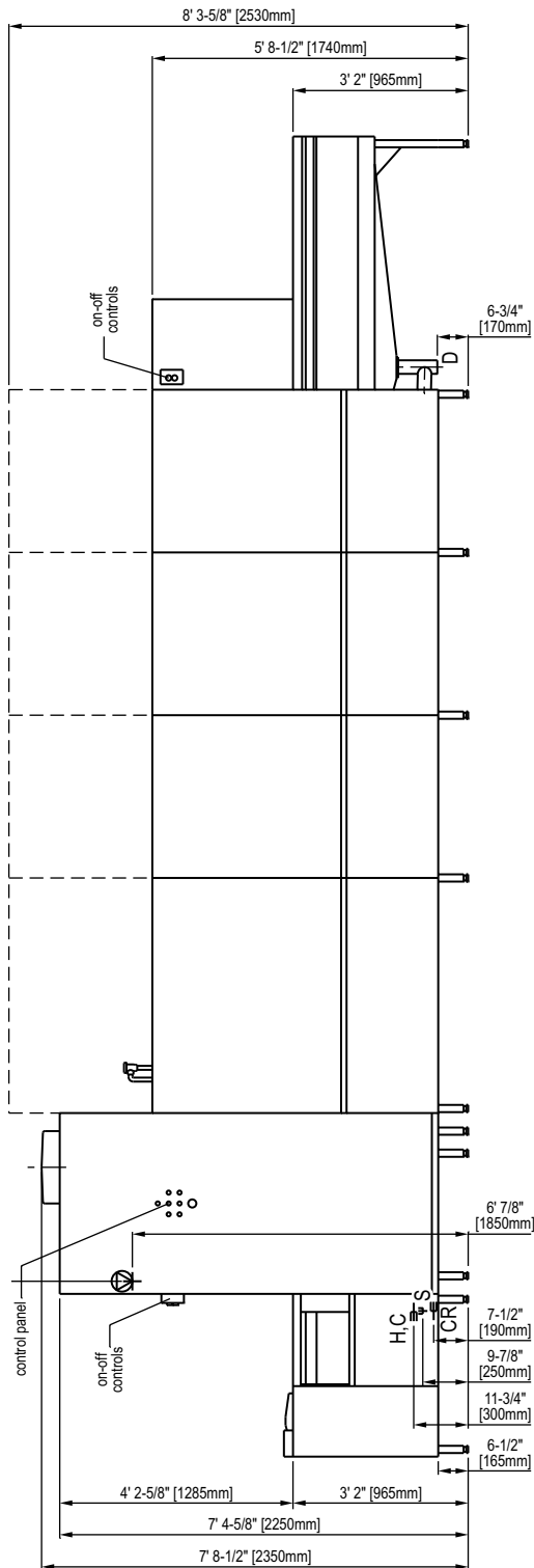
Front Elevation
