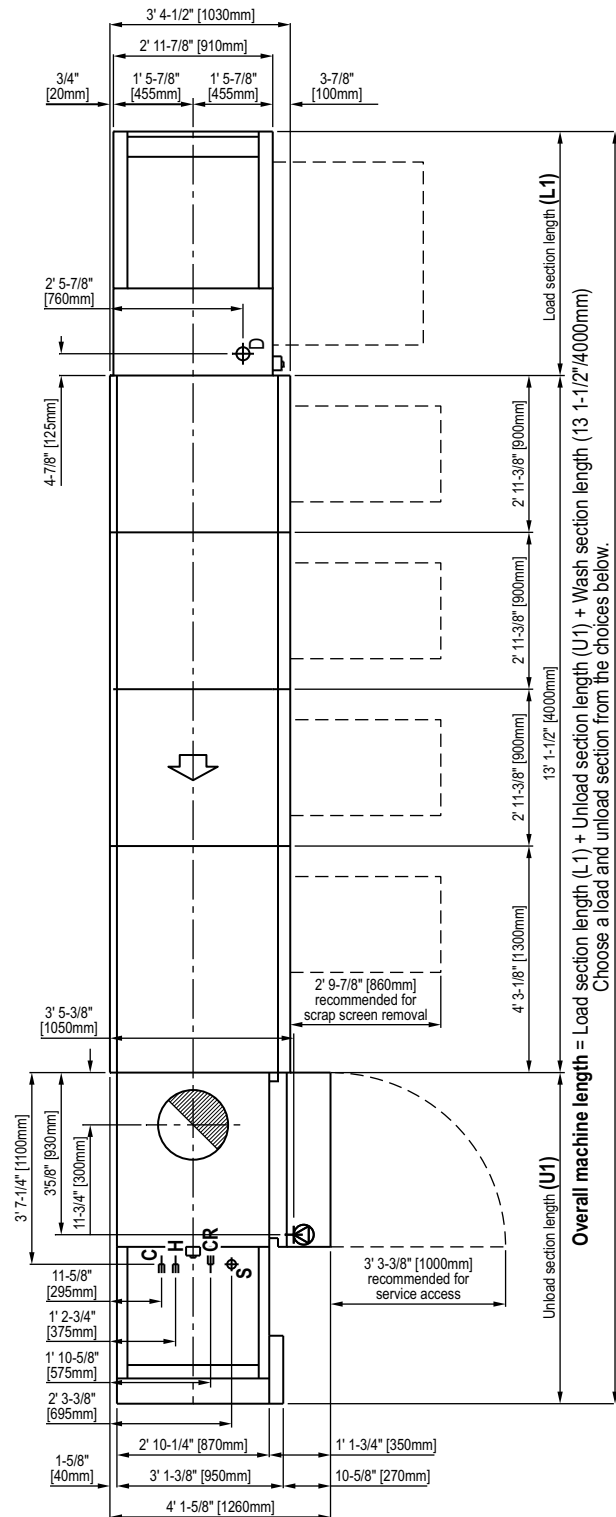
Plan View
