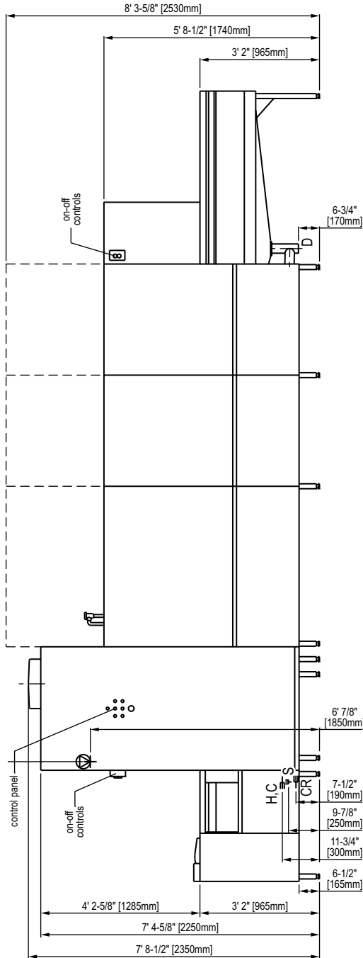
Front Elevation
