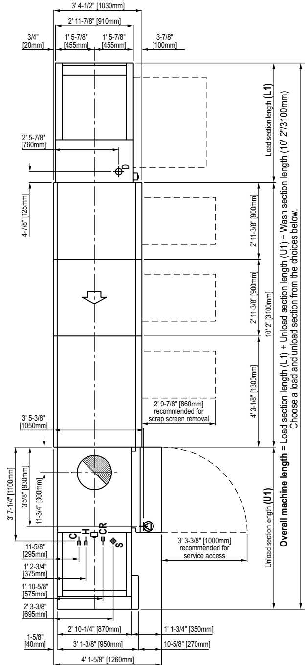
Plan View
