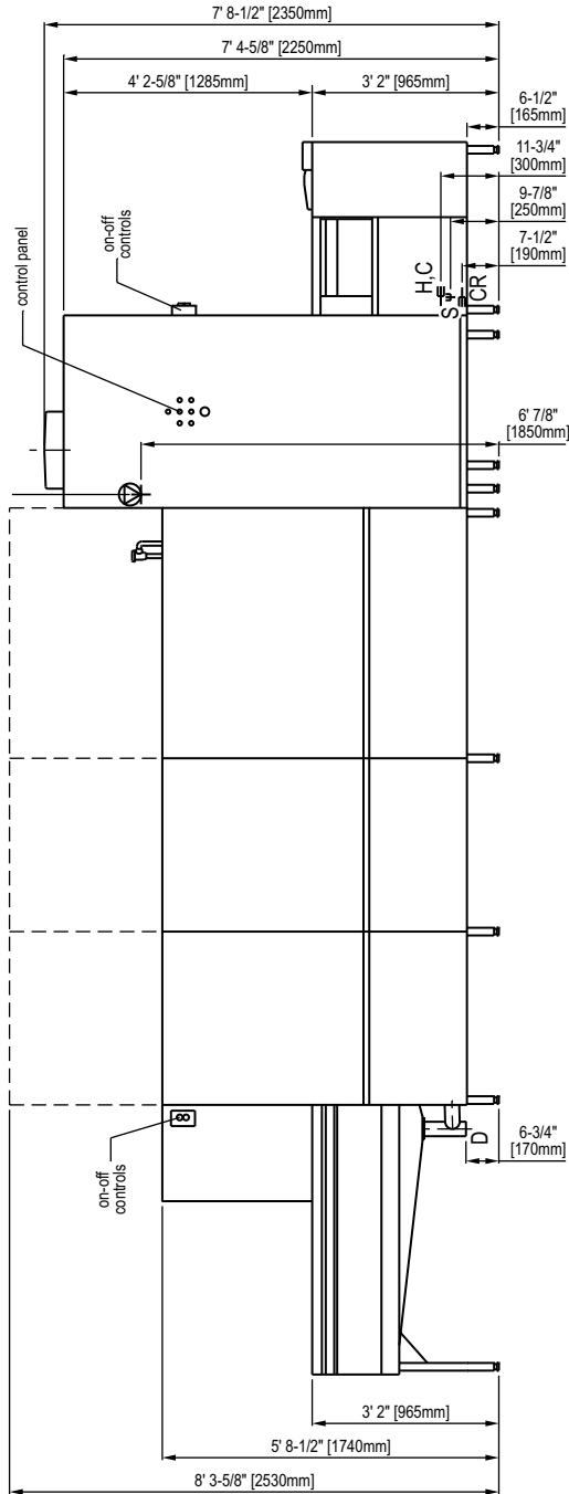
Front Elevation
